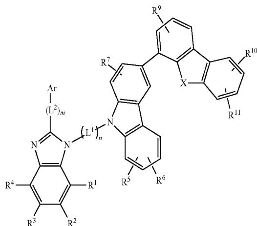
[Chemical Formula 4]
