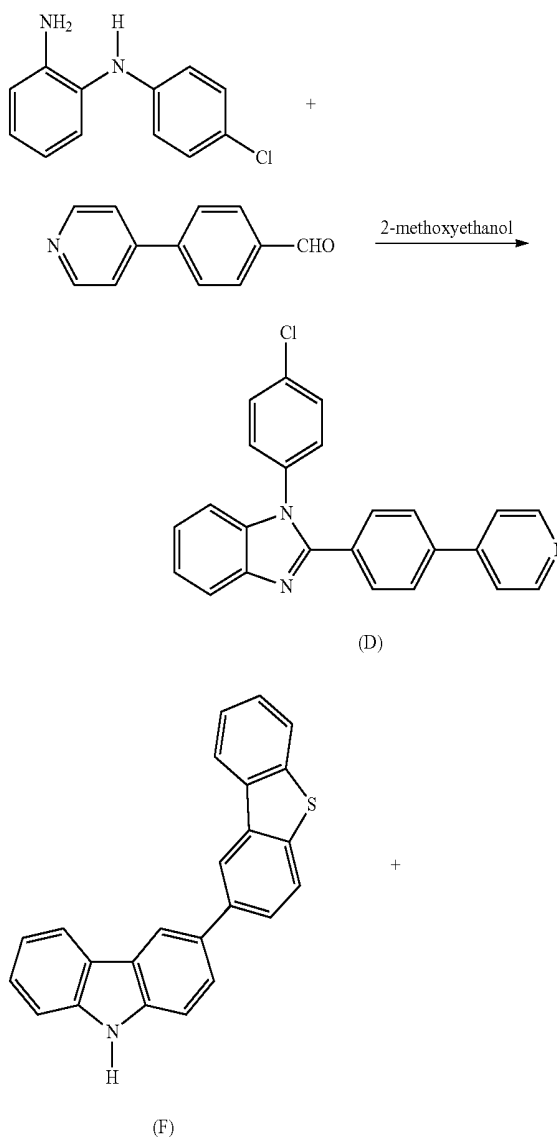
[Reaction Scheme 5]
