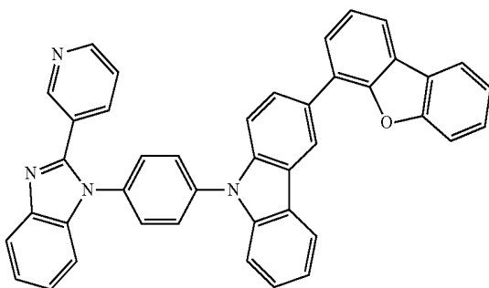
[Chemical Formula [11]]
