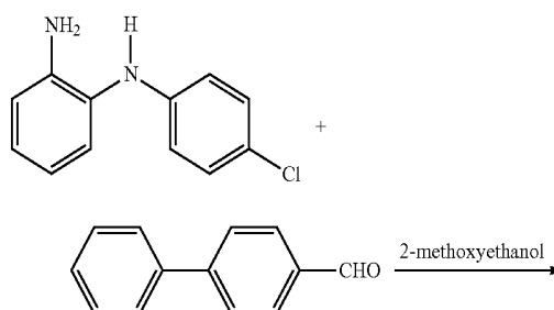
[Reaction Scheme 1]
