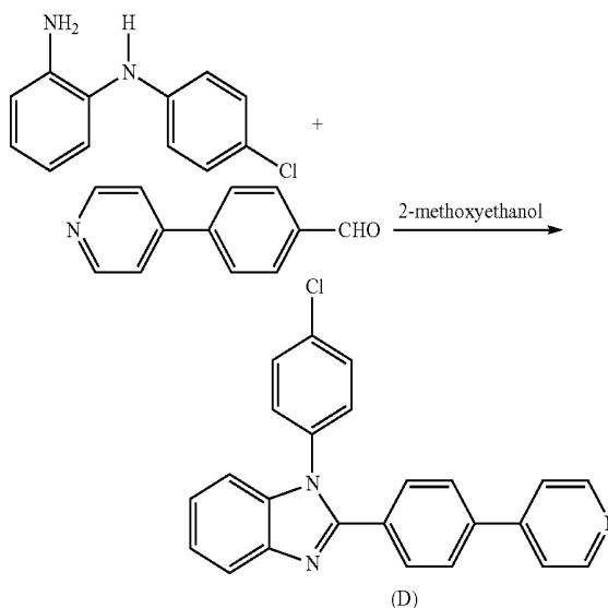
[Reaction Scheme 3]
