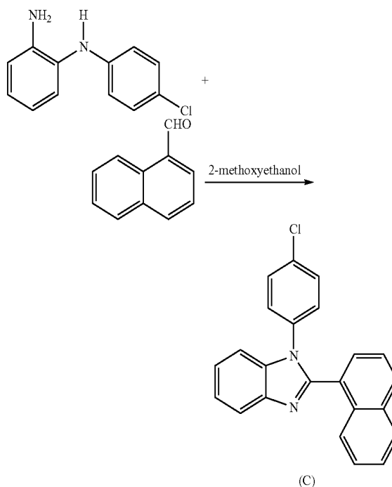
[Reaction Scheme 2]
