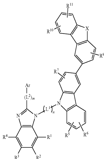
[Chemical Formula 3]
