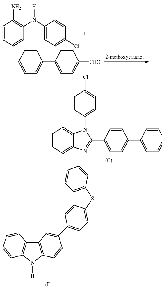
[Reaction Scheme 4]
